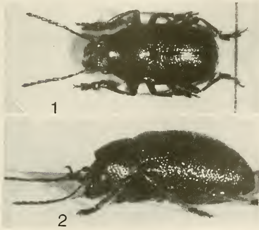
Figures 1-2: Habitus photographs of G. dentatus : (1) dorsal aspect, (2) lateral aspect.
